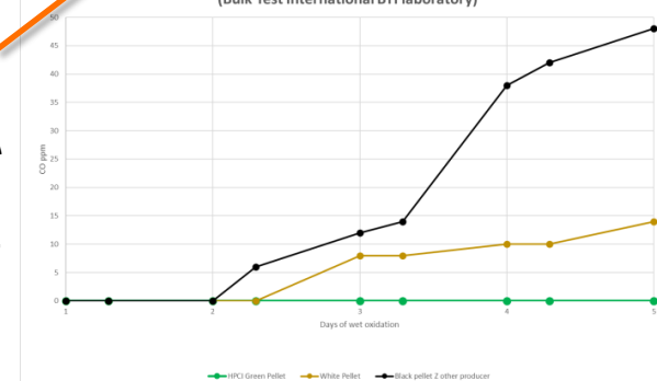
Evolvement of CO (ppm) by day of wet storage (forced oxidation) (Bulk Test International BTI laboratory)
