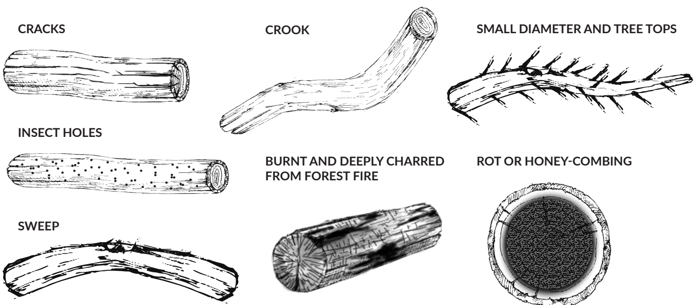
Figure 2 Low-quality logs used for wood pellets
